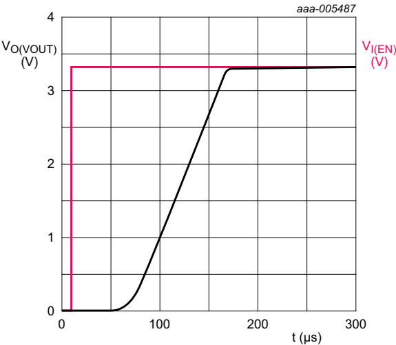
Fig 18. Waveform showing the enable time
