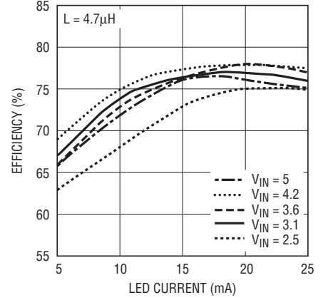
4 LEDs per String Efficiency vs V_{IN} and LED Current
