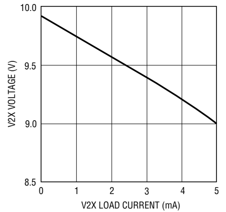
V2X Output Voltage vs V2X Load Current
