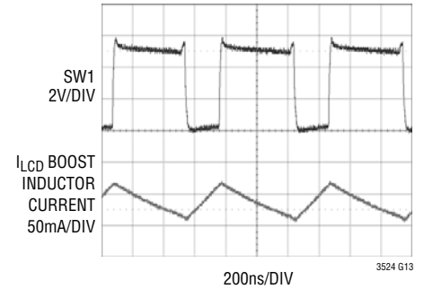
SW1 Voltage and 10 \mu\text{H} Inductor Current at 25mA Load
