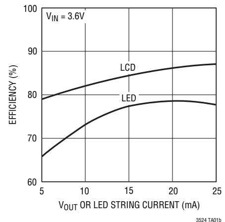
LCD Bias and LED Efficiency V_{IN} = 3.6V , V_{OUT} = 5V , 8 LEDs
