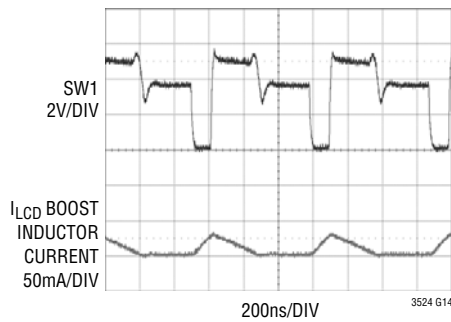
SW1 Voltage and 10 \mu\text{H} Inductor Current at 5mA Load
