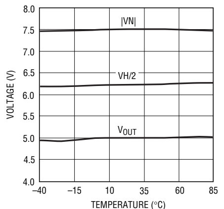
V_{OUT} , |V_N| , and V_H/2 Regulation Overtemperature
