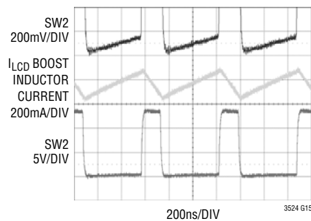
SW2 Voltage and 4.7 \mu\text{H} Inductor Current at 20mA
