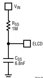
Figure 1. 1ms Soft-Start with 3.6V V_{\text{IN}}
