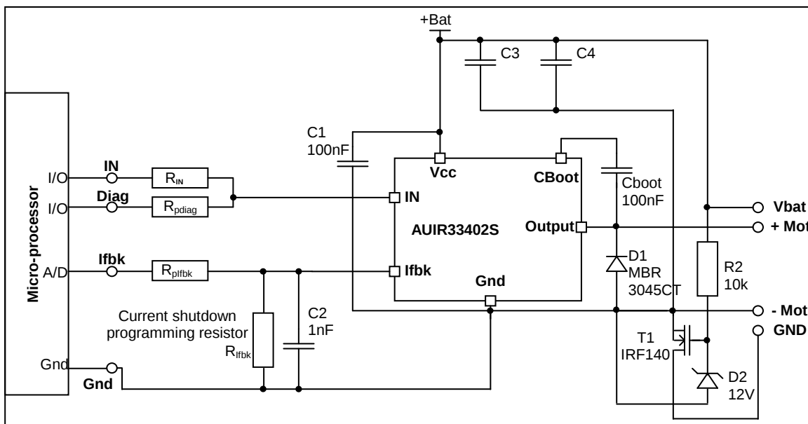
Figure 1: Recommended schematic
