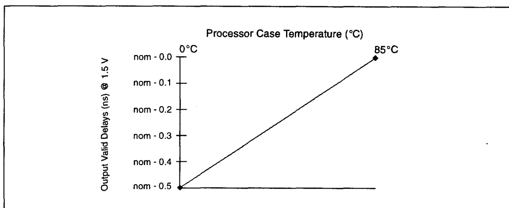
Figure 27. Output Hold Times vs. Temperature
