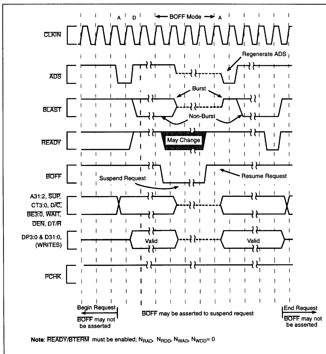
Figure 50. BOFF Functional Timing. BOFF occurs during a burst or non-burst data cycle.
