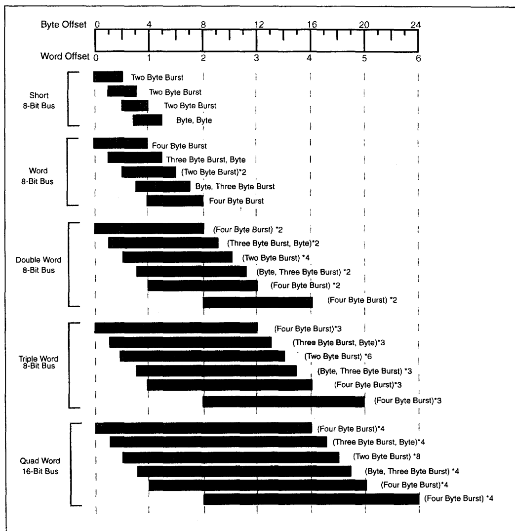
Figure 57. A Summary of Aligned and Unaligned Transfers for 8-Bit Bus
