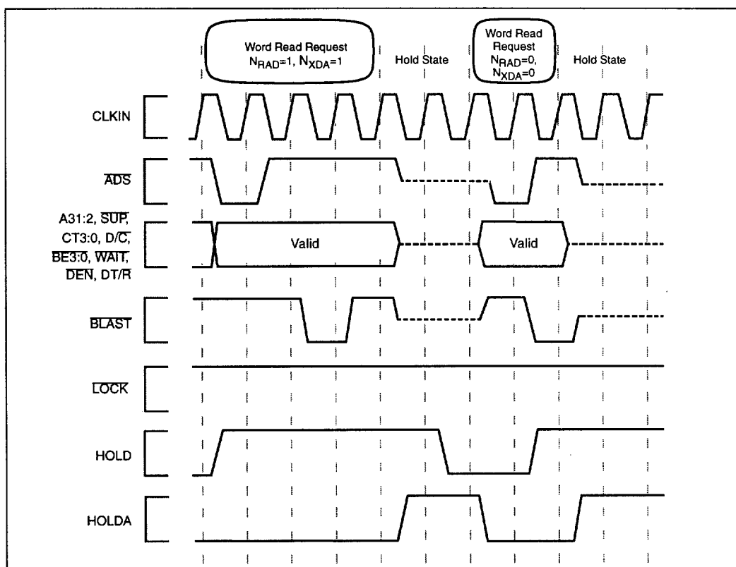
Figure 51. HOLD Functional Timing
