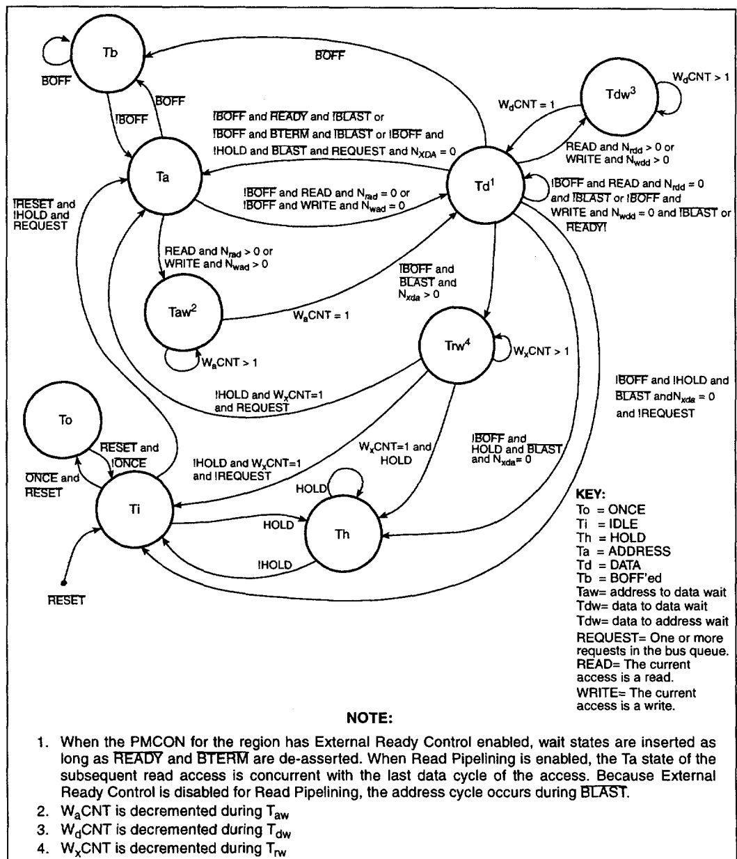
Figure 59. Bus States
