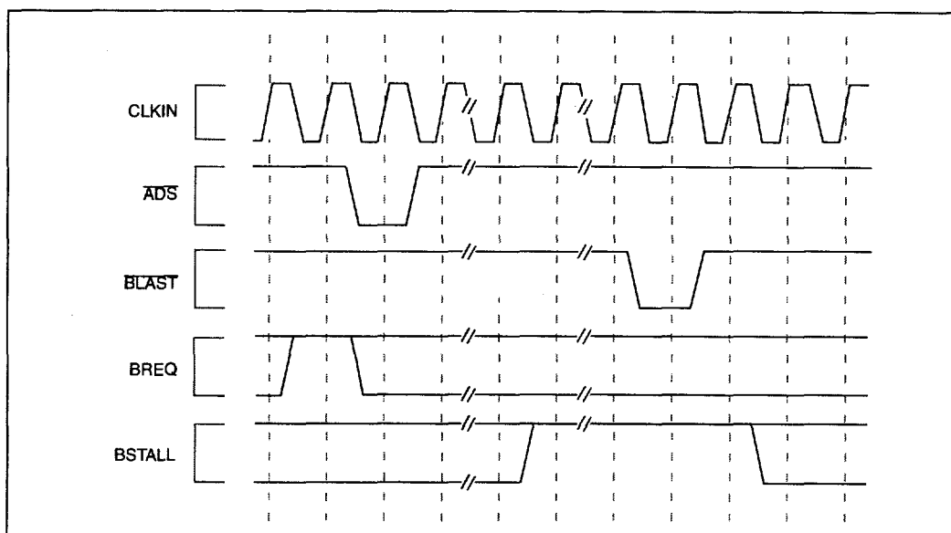
Figure 49. BREQ and BSTALL Operation
