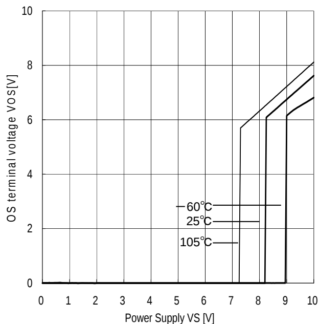
Figure 8 Latch ON supply voltage - Ambient temperature
