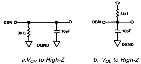
Figure 2. Load Circuits for Data Hold Time Test
