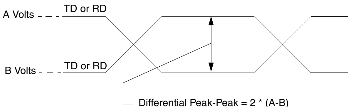
Figure 40. Differential Peak-Peak Voltage of Transmitter or Receiver
