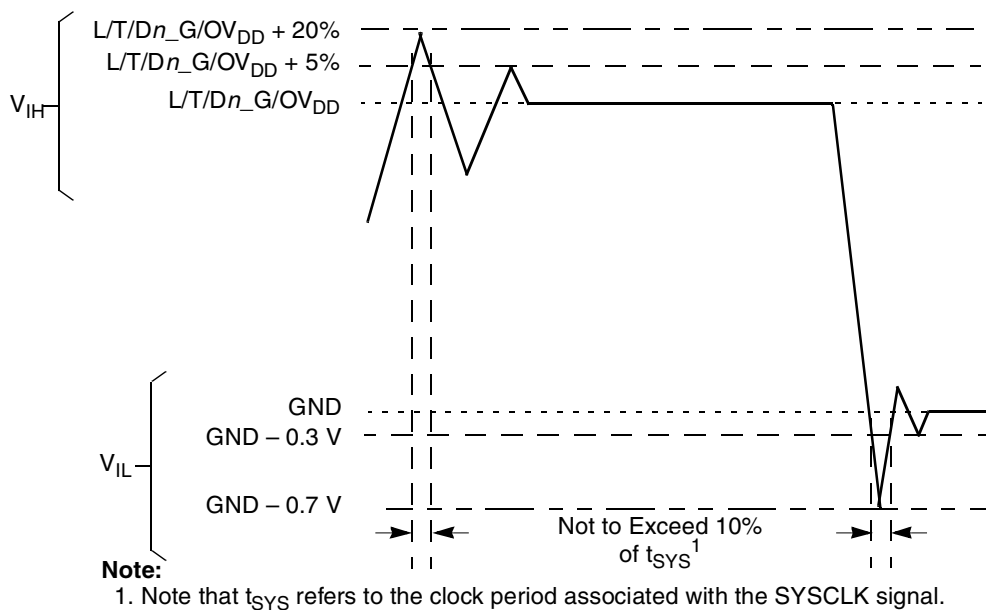
Figure 2. Overshoot/Undershoot Voltage for Dn\_GV_{DD}/OV_{DD}/LV_{DD}
