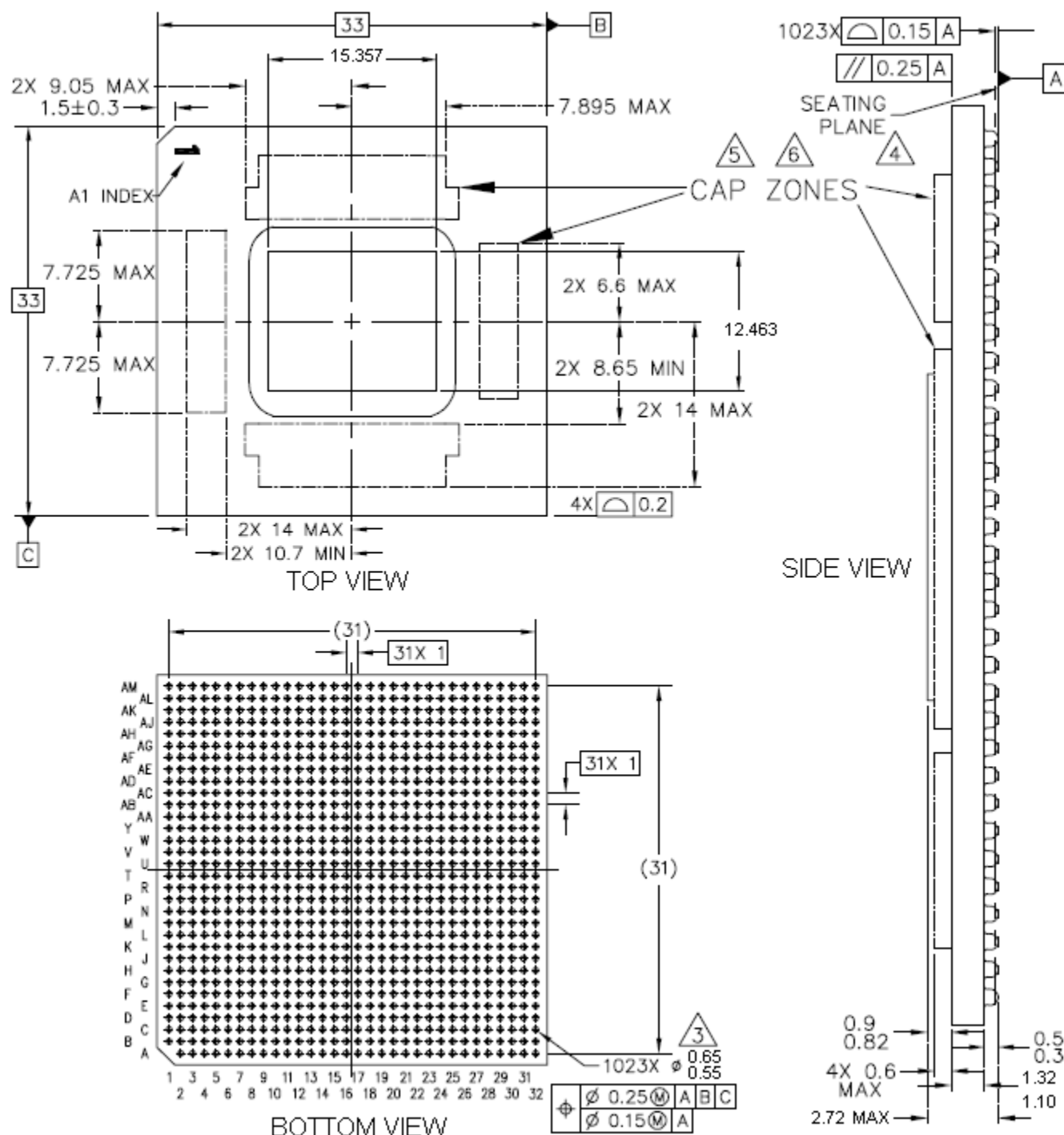
Figure 44. MPC8641 Lead-free or Eutetic Lead FC-CBGA Dimensions
