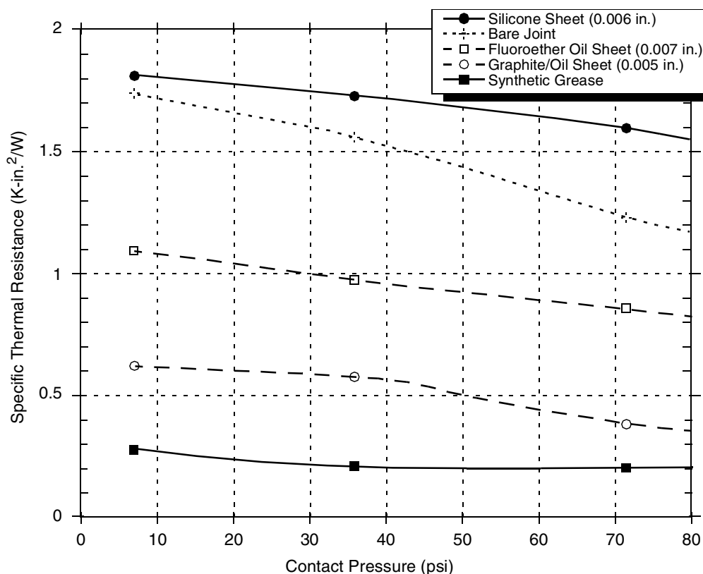
Figure 48. Thermal Performance of Select Thermal Interface Material
