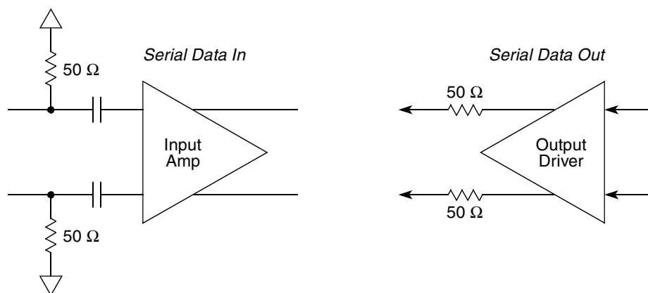
Figure 36. Driver and Receiver of SerDes (PCI Express, Serial RapidIO, and \text{SD\_REF\_CLK}/\overline{\text{SD\_REF\_CLK}} )
