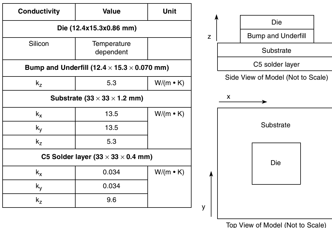
Figure 49. Recommended Thermal Model of MPC8641
