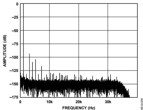
Figure 7. Normal Power Mode; FFT, 1 kHz, -0.5 dB Input Tone, 256× Decimation Rate
