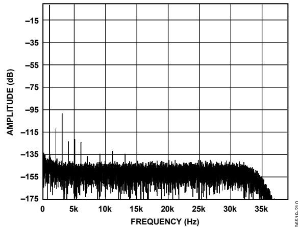
Figure 10. Low Power Mode; FFT, 1 kHz, -0.5 dB Input Tone, 256× Decimation Rate
