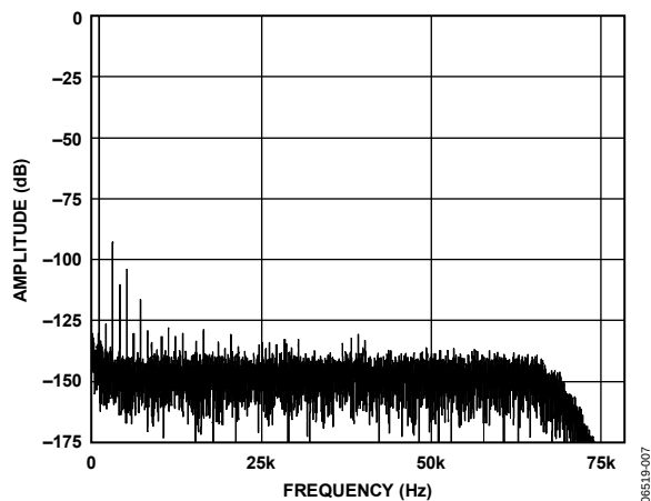
Figure 6. Normal Power Mode; FFT, 1 kHz, -0.5 dB Input Tone, 128× Decimation Rate
