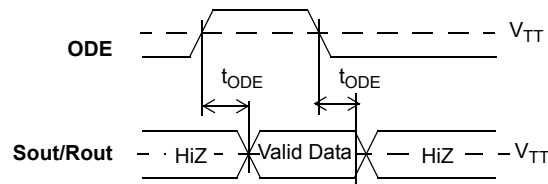
Figure 13 - Output Driver Enable (ODE)
