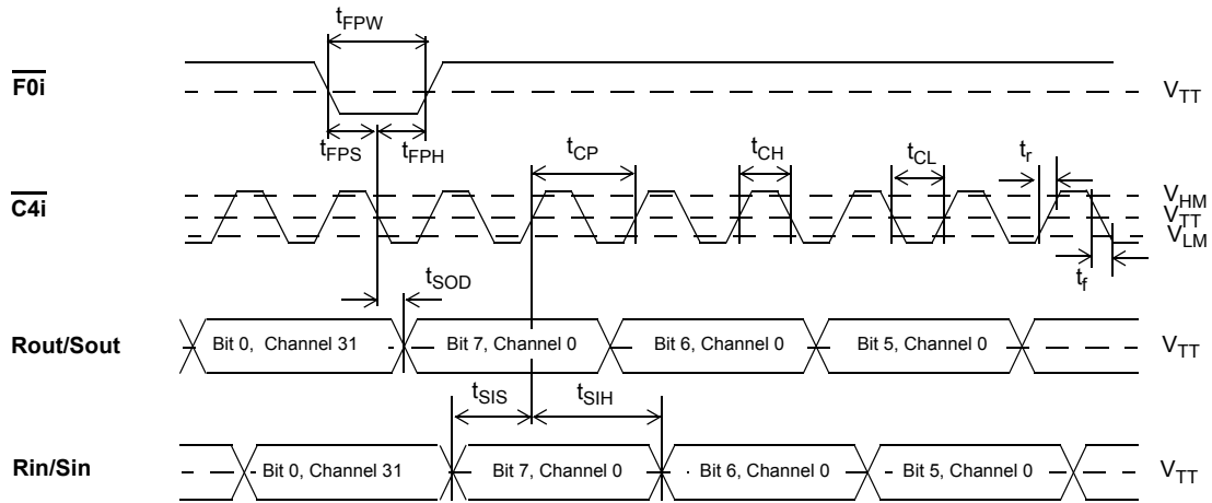
Figure 11 - ST-BUS Timing at 2.048 Mbps
