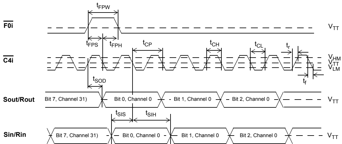
Figure 12 - GCI Interface Timing at 2.048 Mbps
