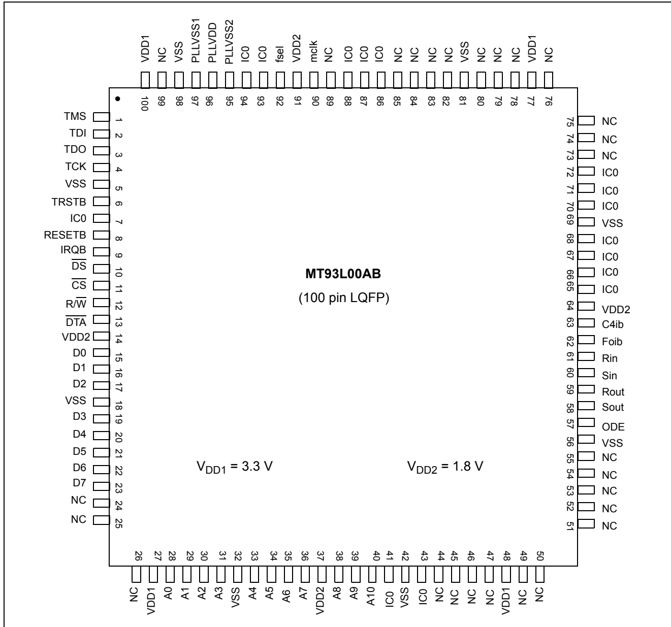
Figure 2 - 100 Pin LQFP
