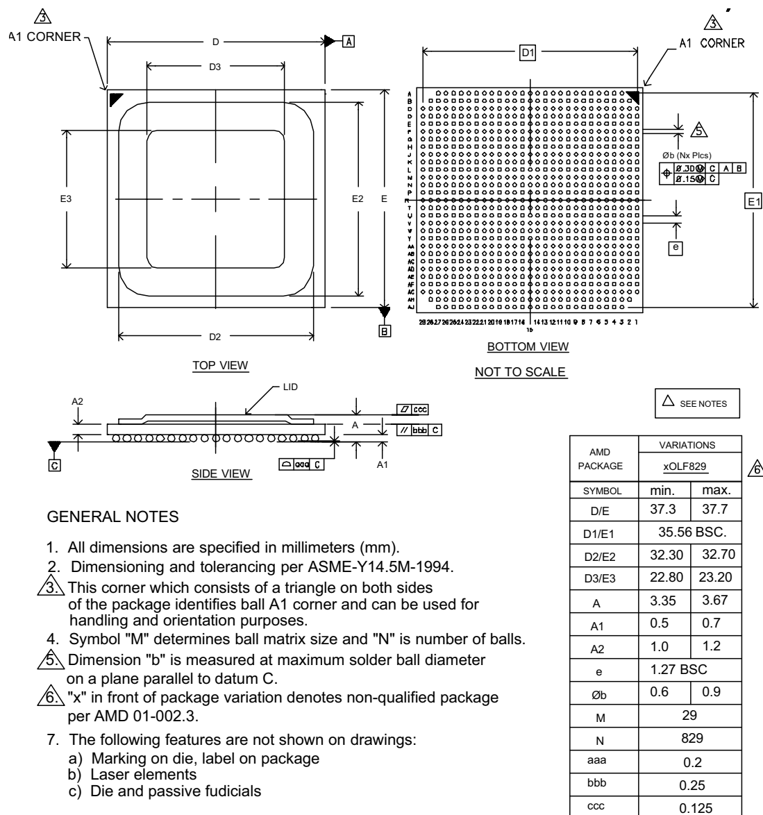
Figure 14: Package mechanical drawing.
