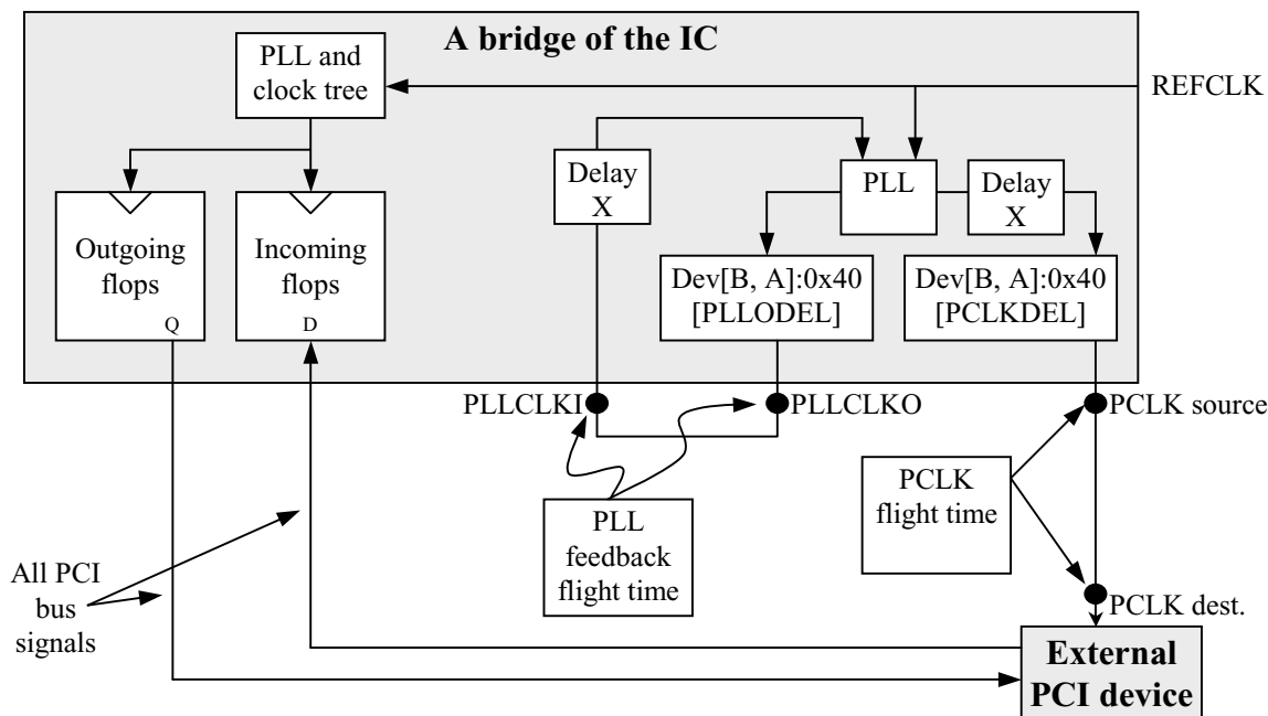
Figure 2: Systemboard clocking.
