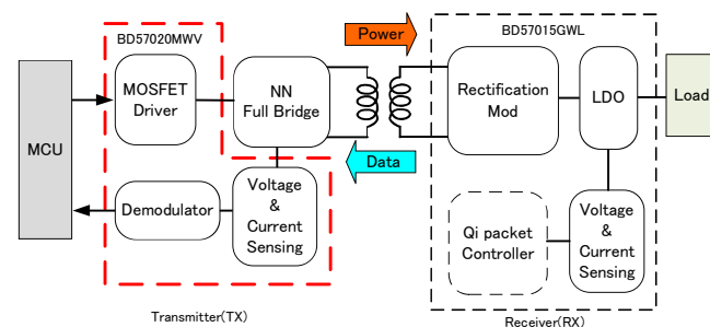
Figure 2. Product position in wireless power supply system
