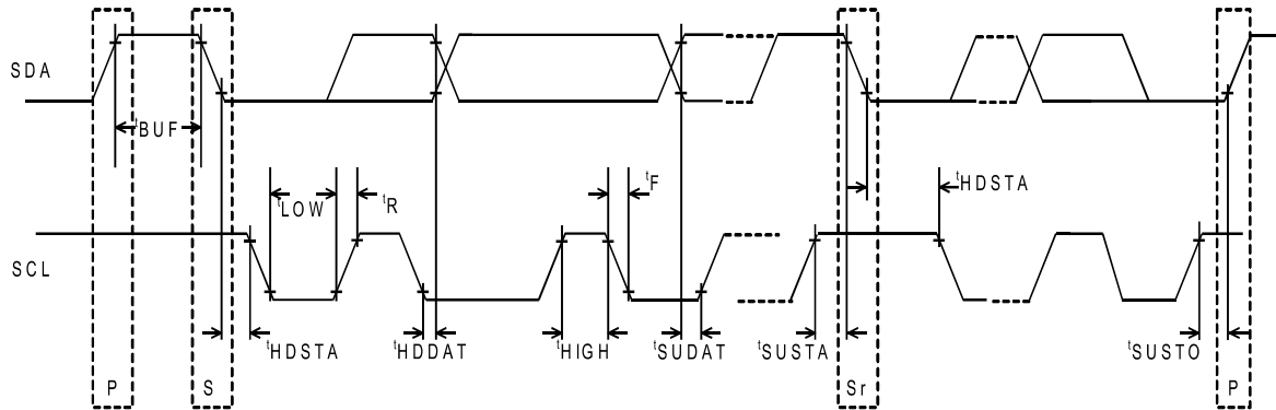
Figure 12. Timing chart
