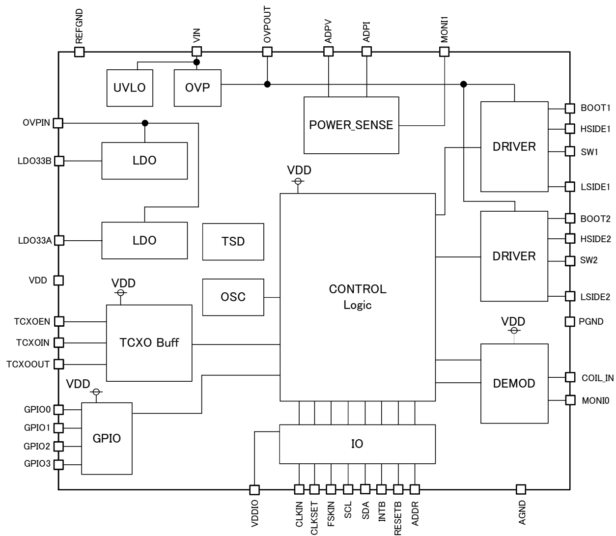
Figure 4. Block diagram
