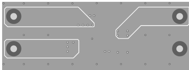
Mid-Layer 2
