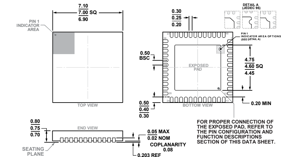
Figure 34. 48-Lead Lead Frame Chip Scale Package [LFCSP] 7 mm × 7 mm Body and 0.75 mm Package Height (CP-48-14) Dimensions shown in millimeters
