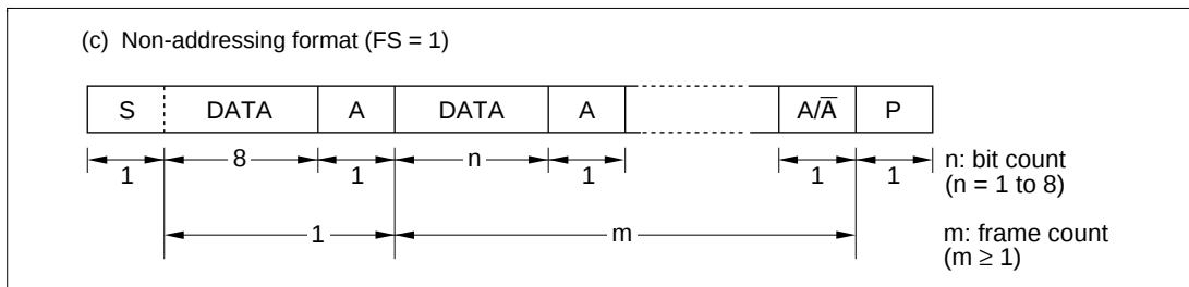
Figure 13.4 I 2 C Bus Data Format (Non-Acknowledge Format)
