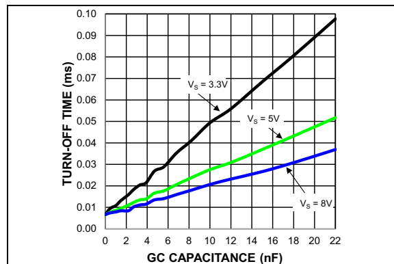
FIGURE 2-5: Turn-Off Time vs. GC Capacitance, V_{IN} = 1.05V .
