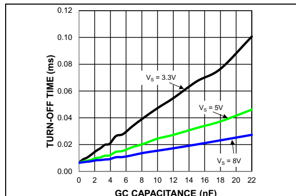
FIGURE 2-6: Turn-Off Time vs. GC Capacitance, V_{IN} = 3.3V .
