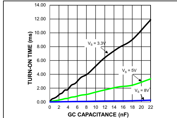
FIGURE 2-4: Turn-On Time vs. GC Capacitance, V_{IN} = 5V .
