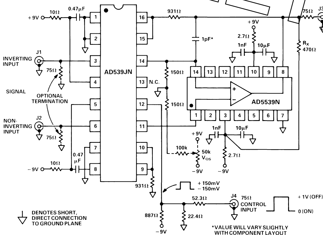
Figure 47. An Analog Multiplier Video Switch
