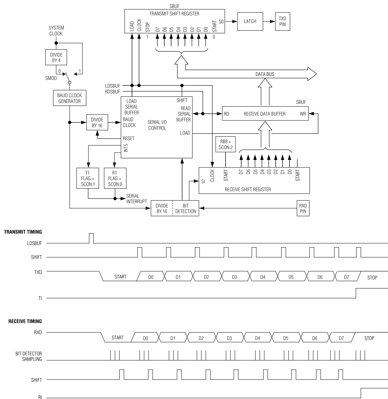
Figure 10-2. UART Mode 1
