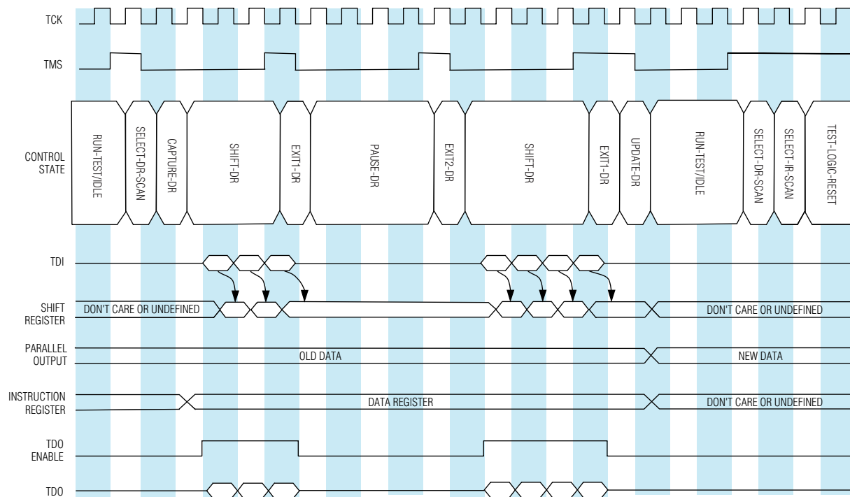
Figure 15-4. TAP Controller Debug Mode DR-Scan Example
