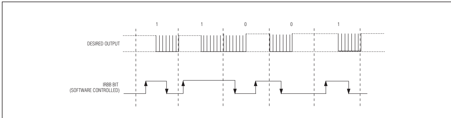
Figure 9-10. Biphase Encoding Example (T2RH Remains Fixed)
