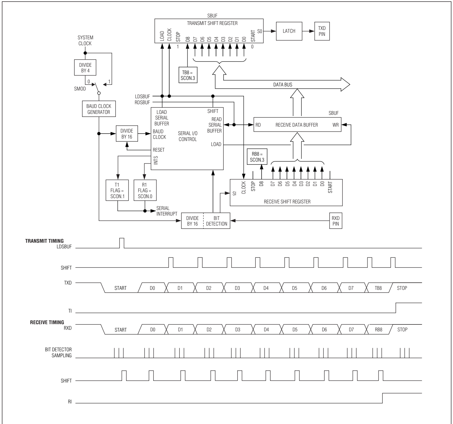
Figure 10-4. UART Mode 3
