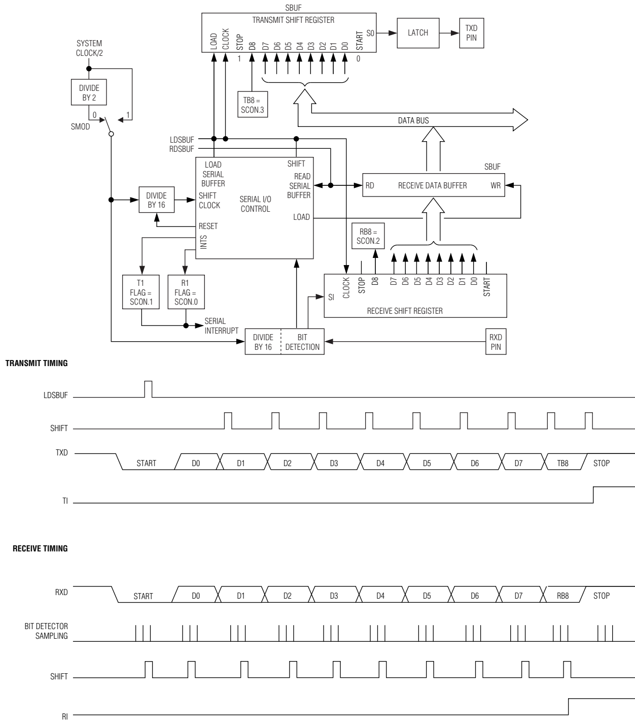
Figure 10-3. UART Mode 2
