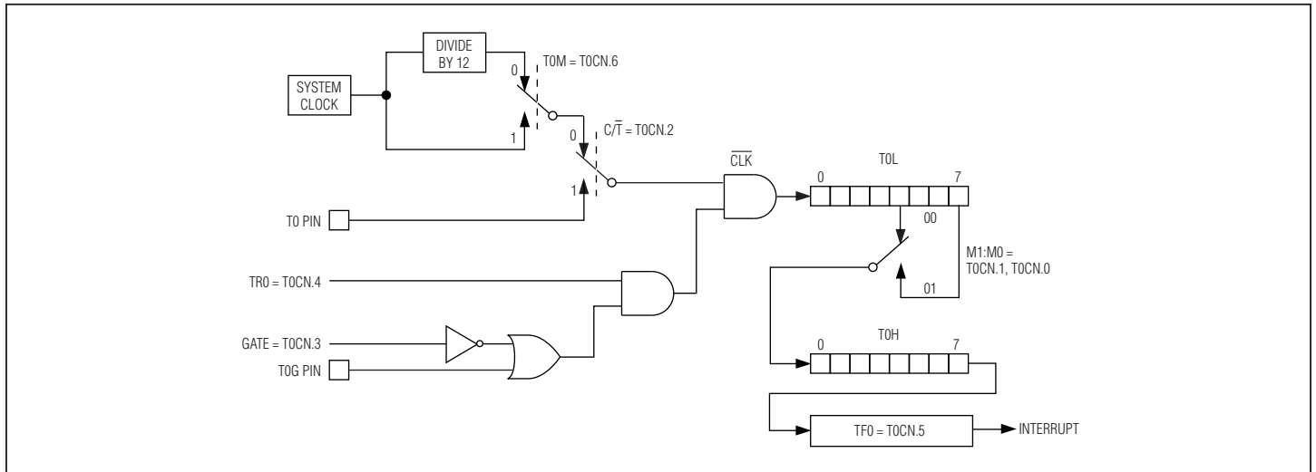
Figure 7-1. Timer/Counter 0 13-Bit/16-Bit Modes
