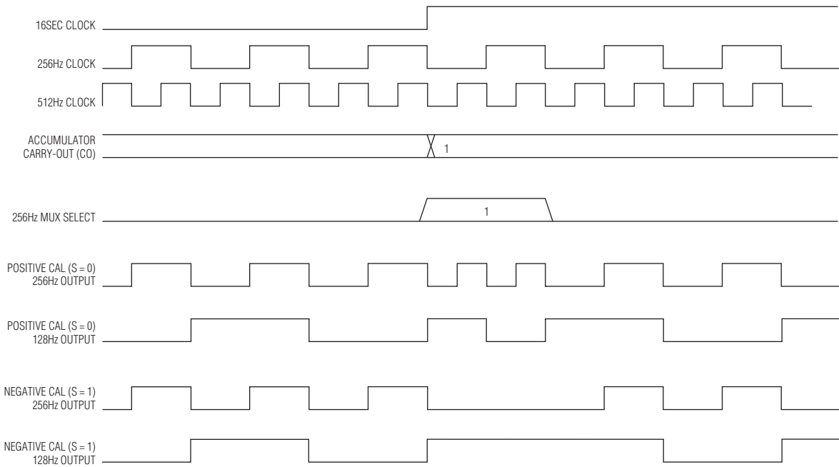
Figure 14-3. Digital Trim Pulse Calibration Diagram
