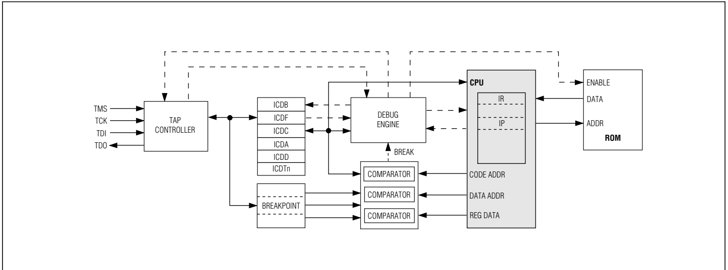
Figure 16-1. In-Circuit Debugger
