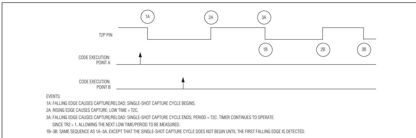
Figure 9-7. Timer 2 Application Example—Measure Duty Cycle
