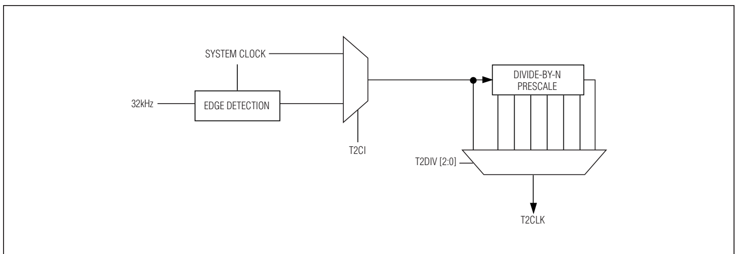
Figure 9-3. Timer 2 Clock
