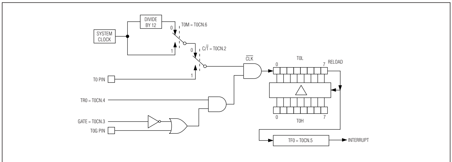
Figure 7-2. Timer/Counter 0 8-Bit Auto-Reload Mode
