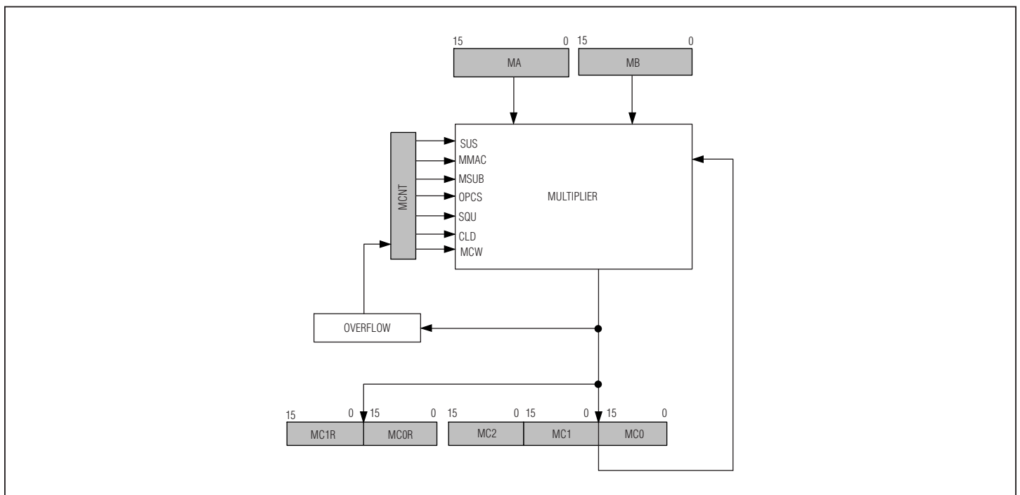
Figure 12-1. Multiplier Organization
