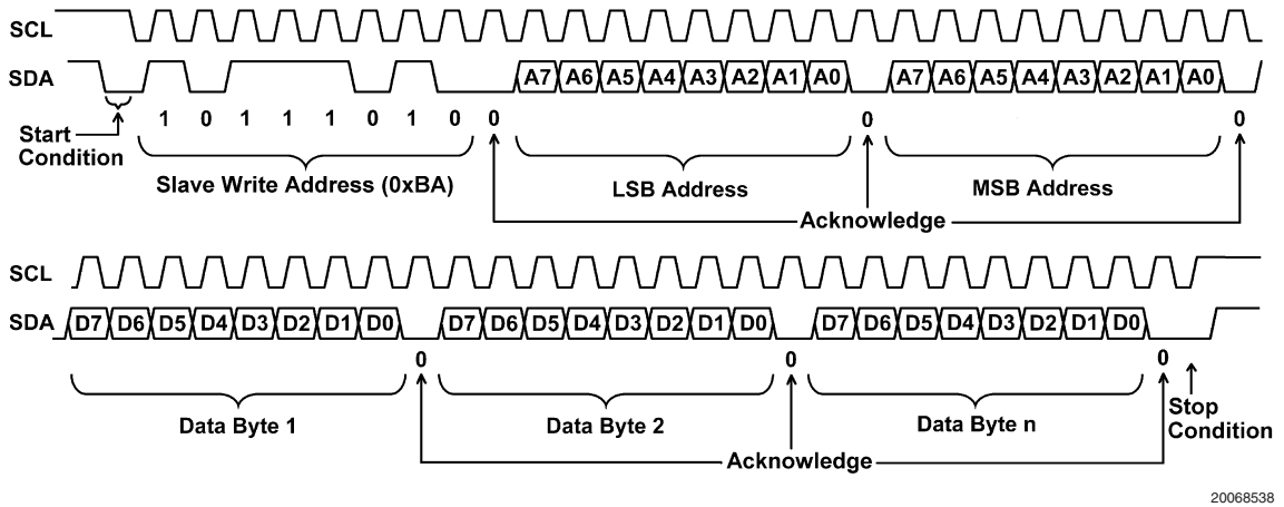
FIGURE 25. I²C Compatible Write Sequence
