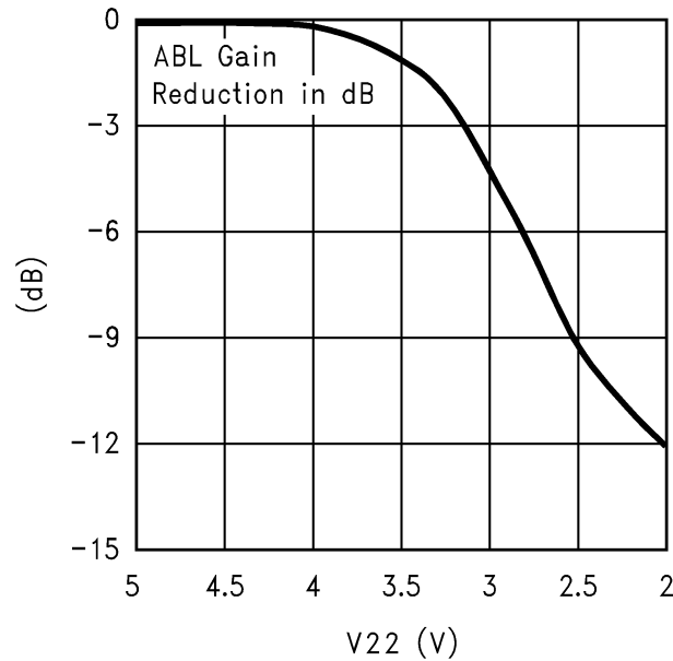
FIGURE 8. ABL Gain Reduction Curve
