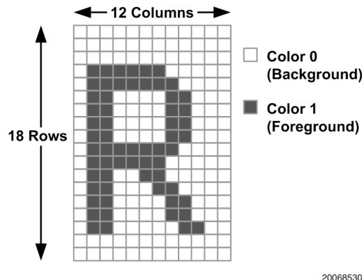
FIGURE 17. Two-Color Character
