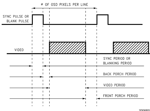
FIGURE 13. Timing Intervals
