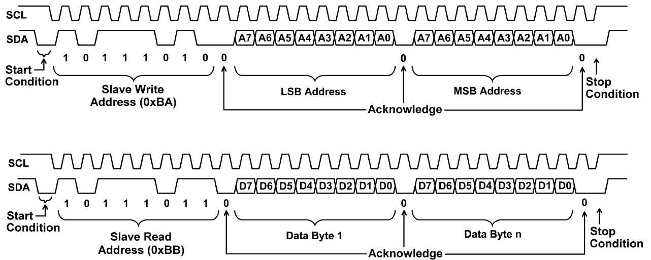
FIGURE 26. I²C Compatible Read Sequence
