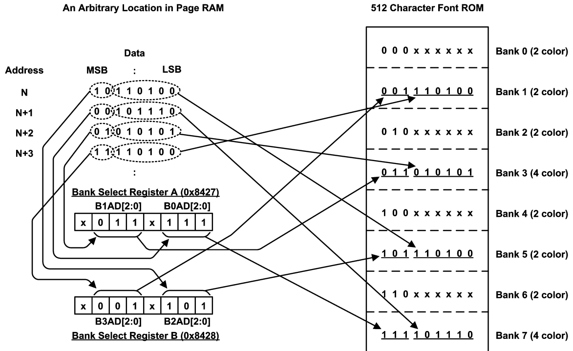
FIGURE 15. Bank Addressing
