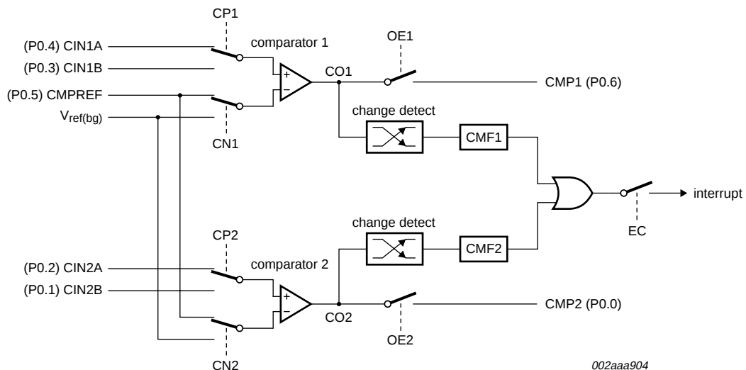
Fig 15. Comparator input and output connections
