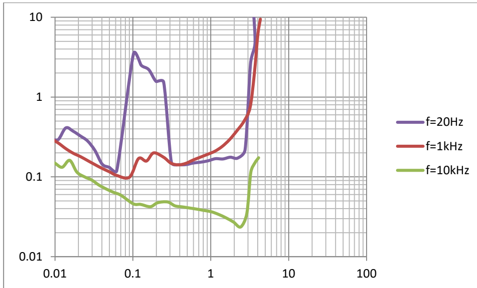
THD+N vs Output Power V_{CC}=8V , R_L= 8\ BTL
