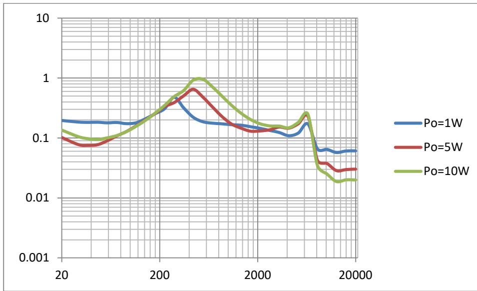
THD+N vs Frequency, V_{CC}=18V , R_L= 8\ BTL
