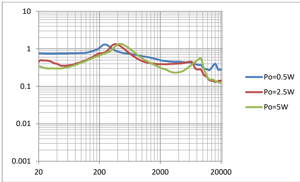
THD+N vs Frequency, Vcc=18V RI=4 SE
