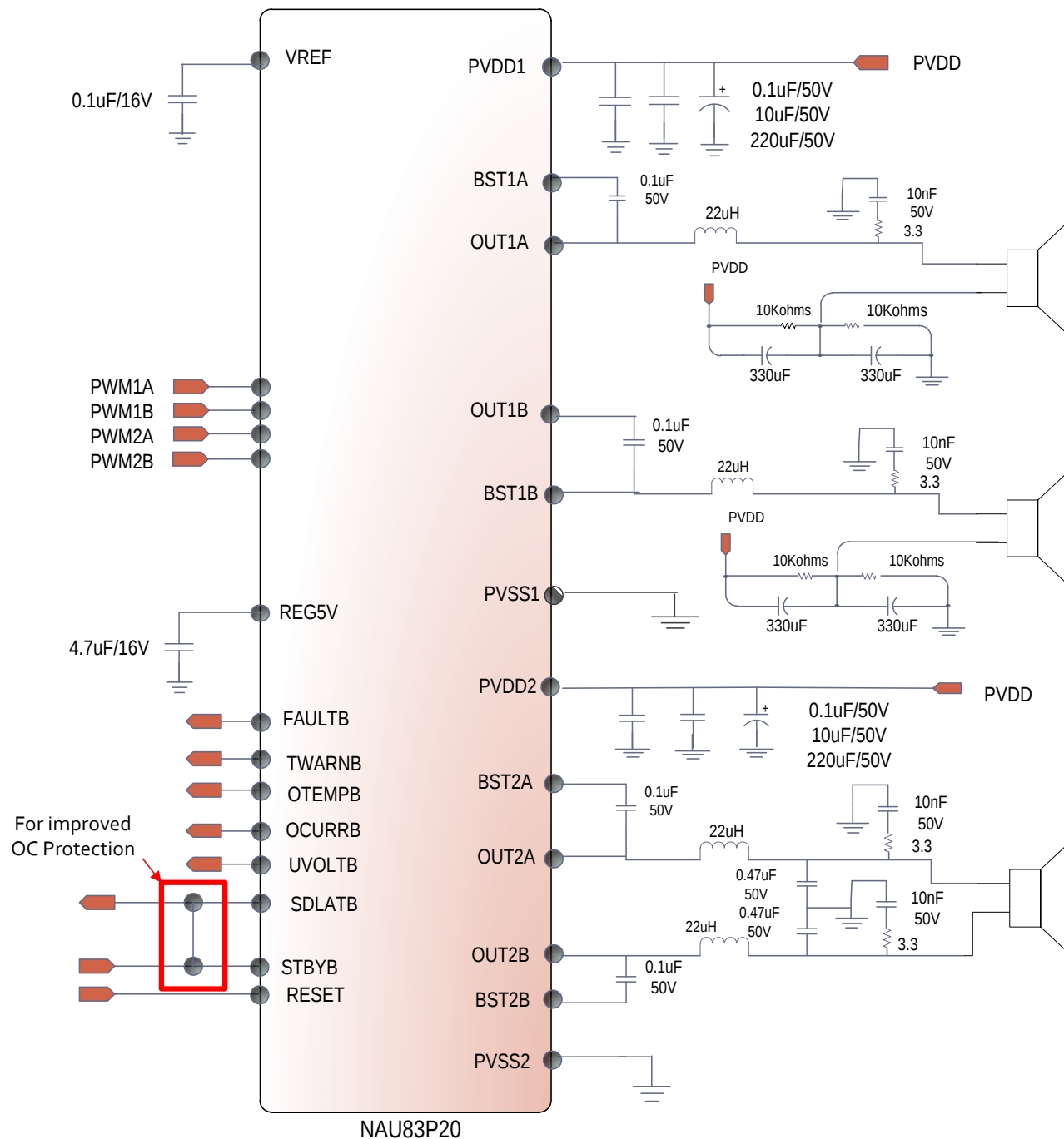
Figure 4: Sub-Woofer Application with Modulation Filters
