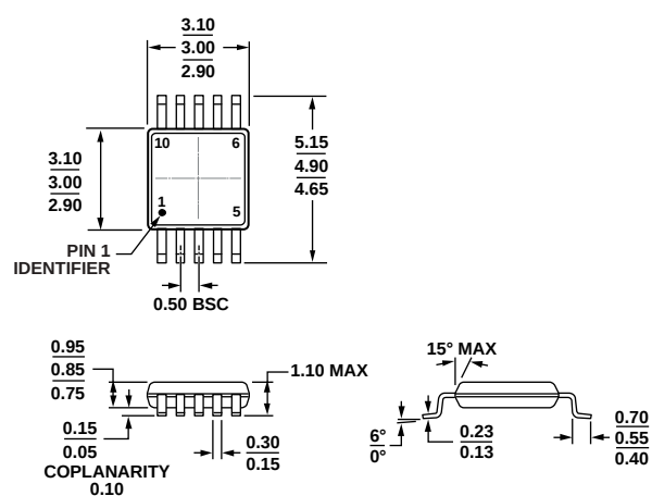
Figure 64. 10-Lead Mini Small Outline Package [MSOP] (RM-10) Dimensions shown in millimeters
