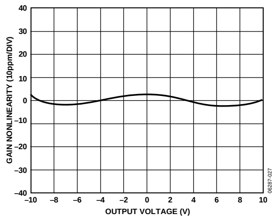
Figure 26. Gain Nonlinearity vs. Output Voltage, G = 8 , R_L = 10\text{ k}\Omega , 2\text{ k}\Omega , 600\text{ }\Omega
