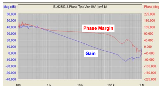
FIGURE 53. REFERENCE DESIGN LOOP GAIN T2(s) MEASUREMENT RESULT
