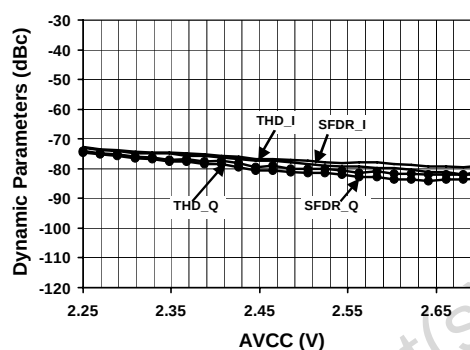
Figure 12. Distortion vs. AV_{CC} F_S=20\text{Mpsps} ; I_{CCA}=40\text{mA} ; F_{in}=5\text{MHz}
