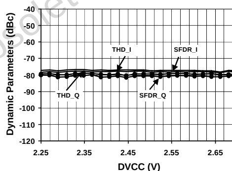
Figure 14. Distortion vs. DV_{CC} F_S=20\text{Mpsps} ; I_{CCA}=40\text{mA} ; F_{in}=5\text{MHz}
