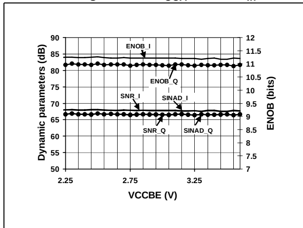
Figure 17. Linearity vs. V_{CCBE} F_S=20\text{Mpsps} ; I_{CCA}=40\text{mA} ; F_{in}=5\text{MHz}
