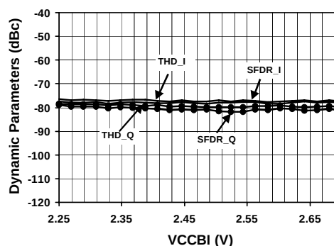
Figure 16. Distortion vs. V_{CCBI} F_S=20\text{Mpsps} ; I_{CCA}=40\text{mA} ; F_{in}=5\text{MHz}
