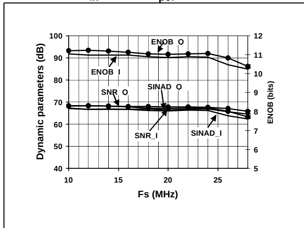
Figure 5. Linearity vs. F_S F_{in}=5\text{MHz} ; R_{pol} adjustment
