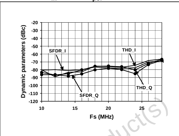
Figure 6. Distortion vs. F_S F_{in}=5\text{MHz} ; R_{pol} adjustment
