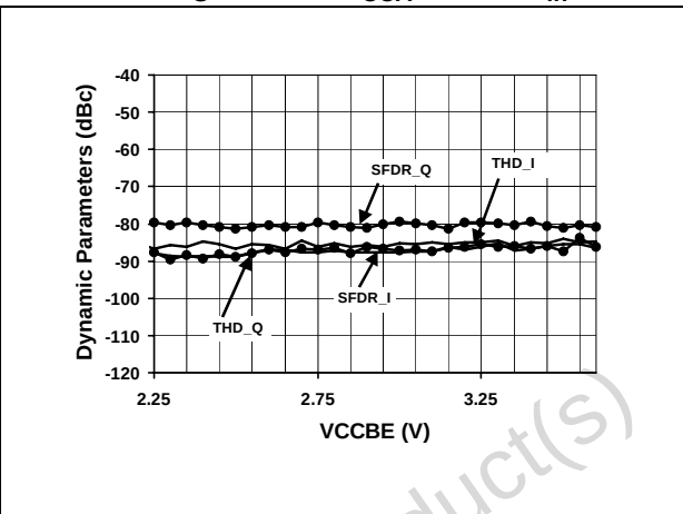
Figure 18. Distortion vs. V_{CCBE} F_S=20\text{Mpsps} ; I_{CCA}=40\text{mA} ; F_{in}=5\text{MHz}
