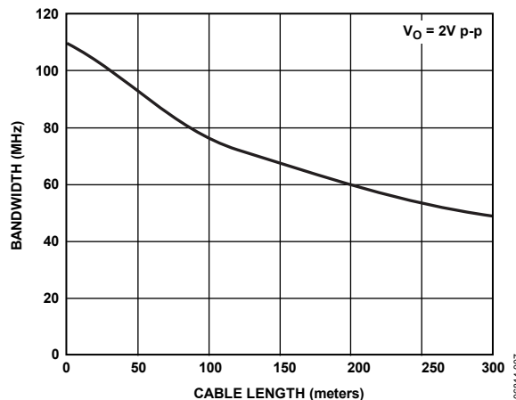
Figure 9. Equalized -3 dB Bandwidth vs. Cable Length
