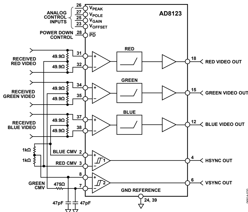
Figure 20. Basic Application Circuit with Common-Mode Sync Extraction
