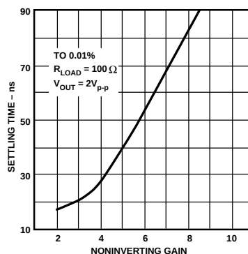
Figure 17. Settling Time vs. Noninverting Gain
