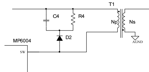
Figure 11: RCD snubber
