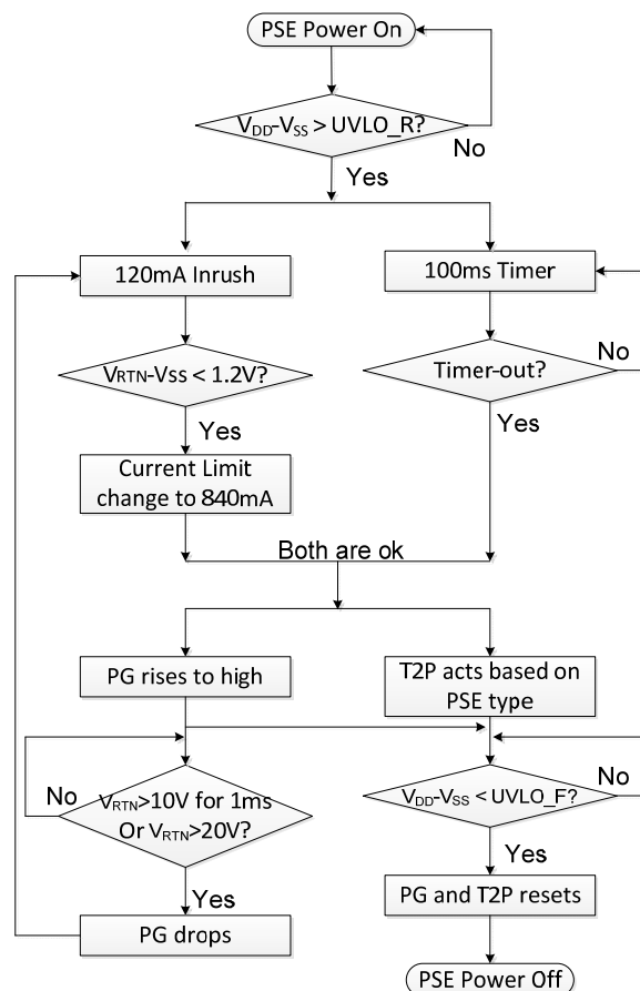
Figure 3: Startup Sequence
