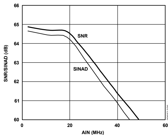
Figure 30. Measured SNR and SINAD (Encode = 105 MSPS)
