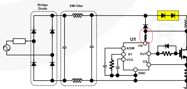
Figure 6. High-Voltage Application
