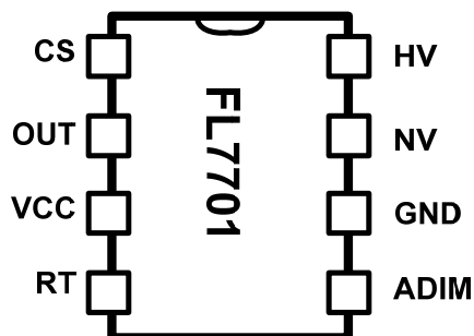
Figure 3. Pin Configuration
