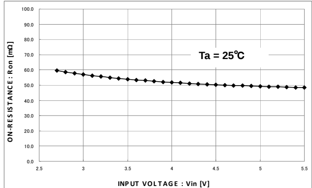
Fig.18 NMOS on resistance-power-supply voltage
