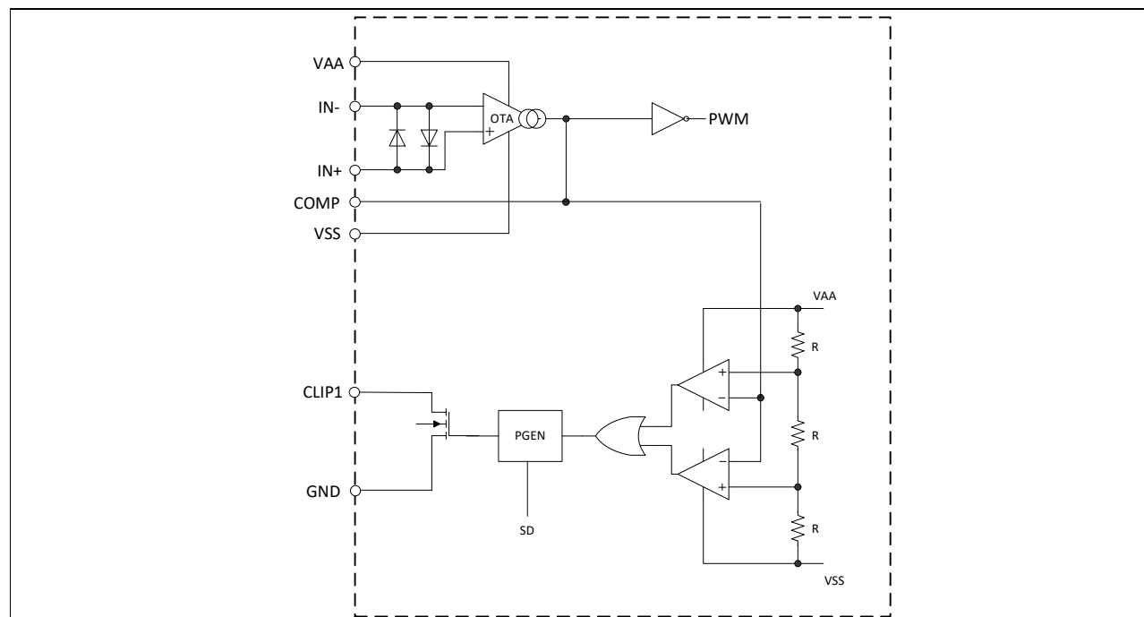
Figure 43 CLIP Detection
