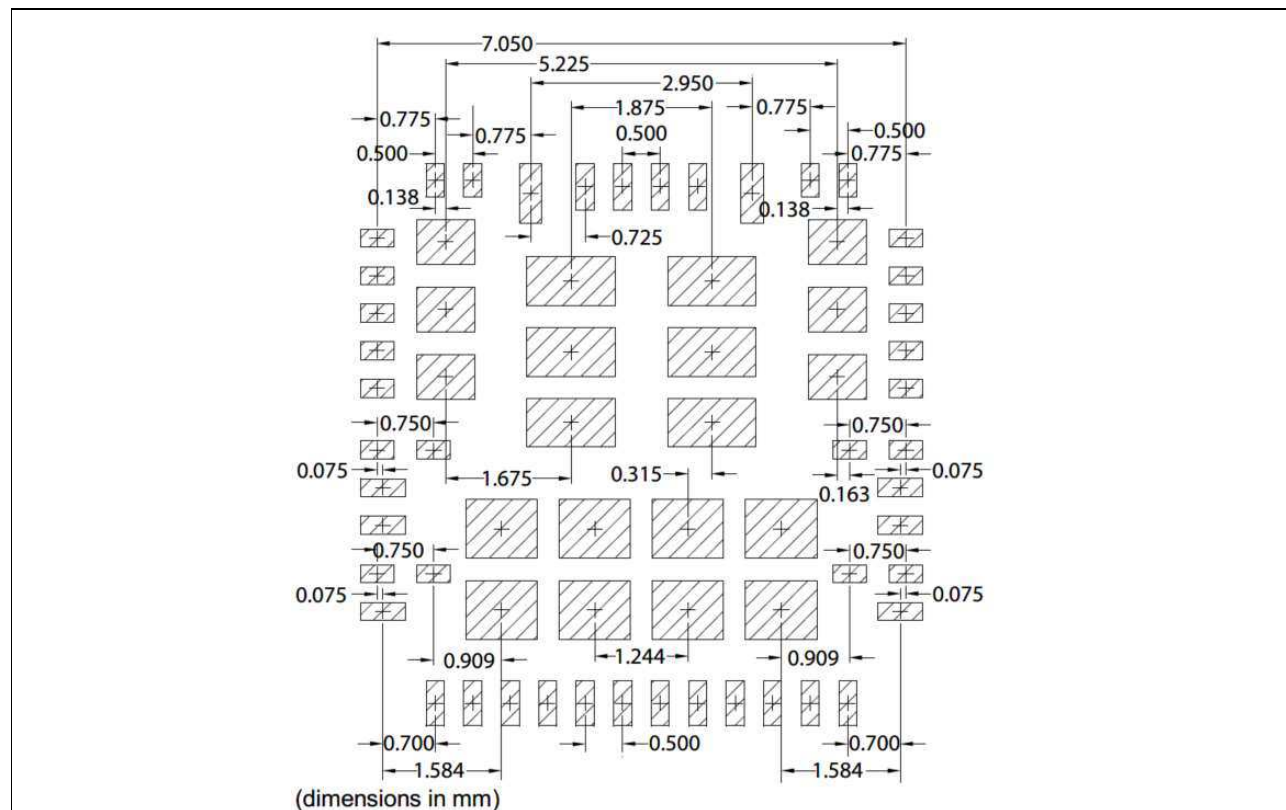
Figure 55 42-lead 7x7 stencil design_1
