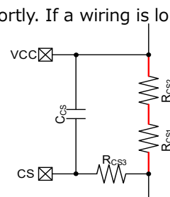
Figure 18. The case of R_{CS} Series
