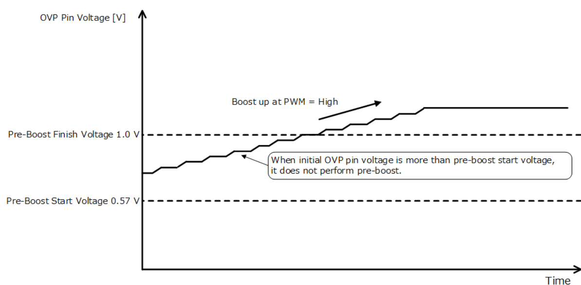
Figure 20. Without Pre-boost
