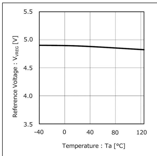
Figure 7. Reference Voltage vs Temperature ( V_{CC} = 12\text{ V} to 35\text{ V} , V_{EN} = 3.3\text{ V} , V_{PWM} = 5\text{ V} )
