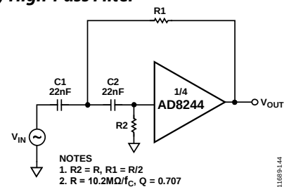
Figure 43. Sallen-Key High-Pass Filter
