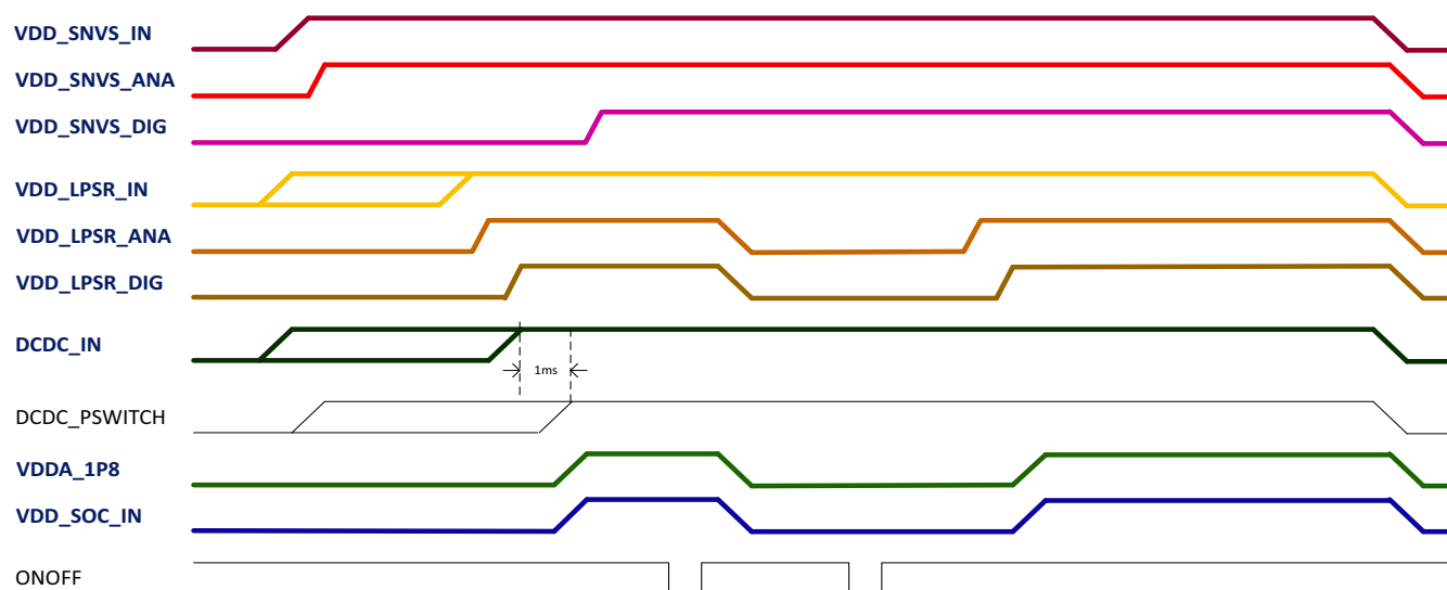
Figure 4. Power sequence
