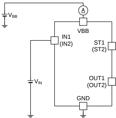
Figure 32. Operating Current
