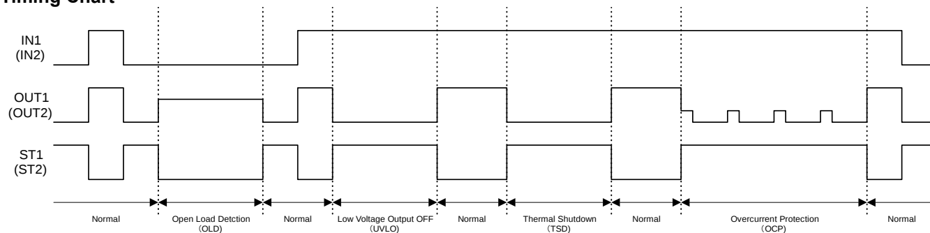
Figure 43. Timing Chart
