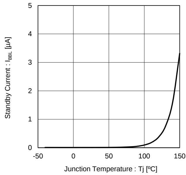
Figure 12. Standby Current vs Junction Temperature
