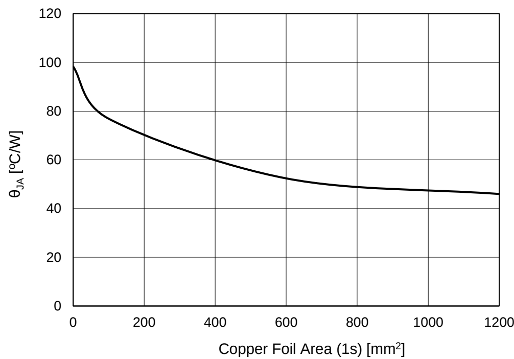
Figure 10. Thermal Resistance
