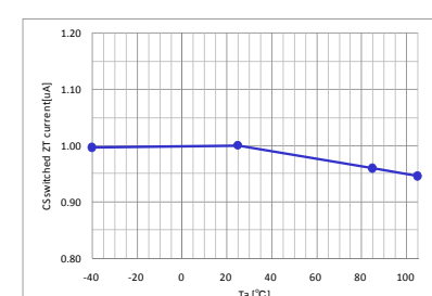
Fig-47-38 CS switched ZT current
