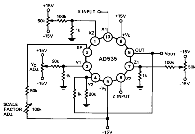
Figure 6. Precision Divider with Four External Adjustments
