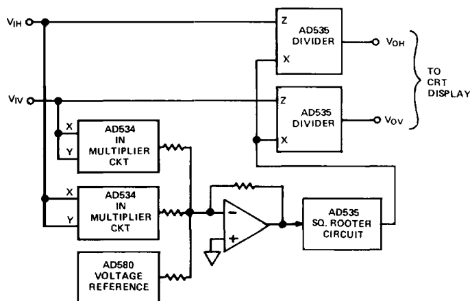
Figure 8. Pin-Cushion Corrector
