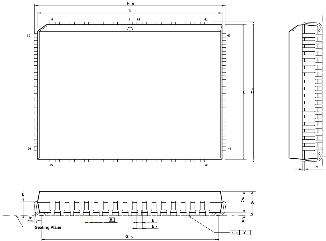
68 pin PLCC
