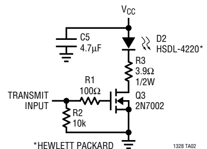
IrDA Transmitter
