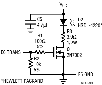
IrDA Transmitter
