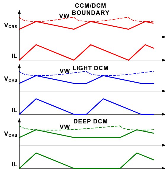
FIGURE 11. PERIOD STRETCHING
