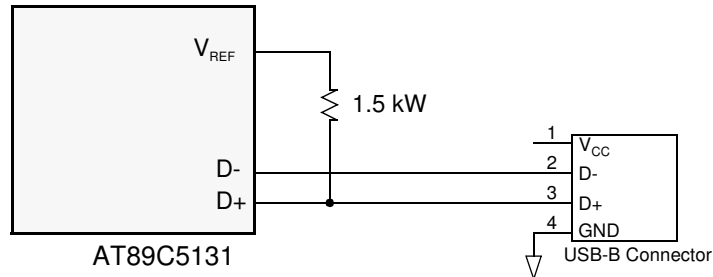
Figure 21-13. Example of V_{REF} Connection
