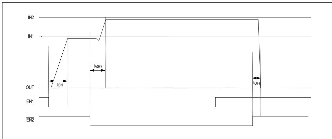
Figure 2: Automatic Switch Operation: \overline{EN2} On (Time scale is exaggerated for easy recognition in the waveform)
