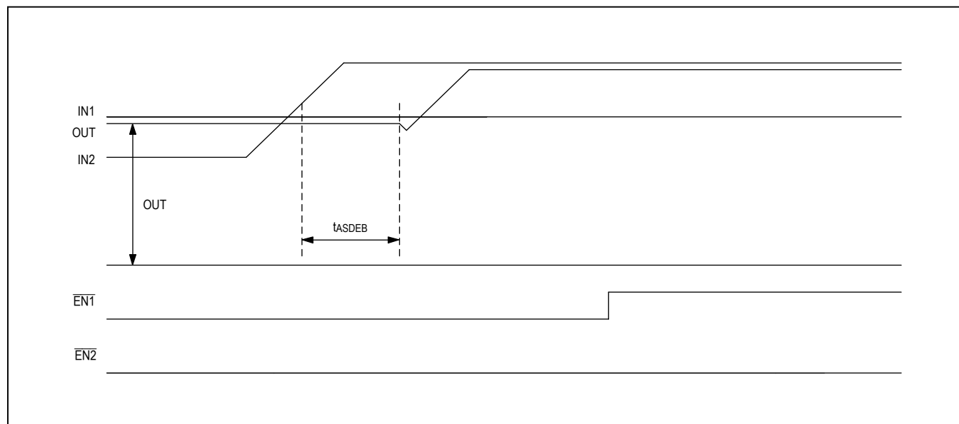
Figure 1. Automatic Switch Operation: IN2 Rise
