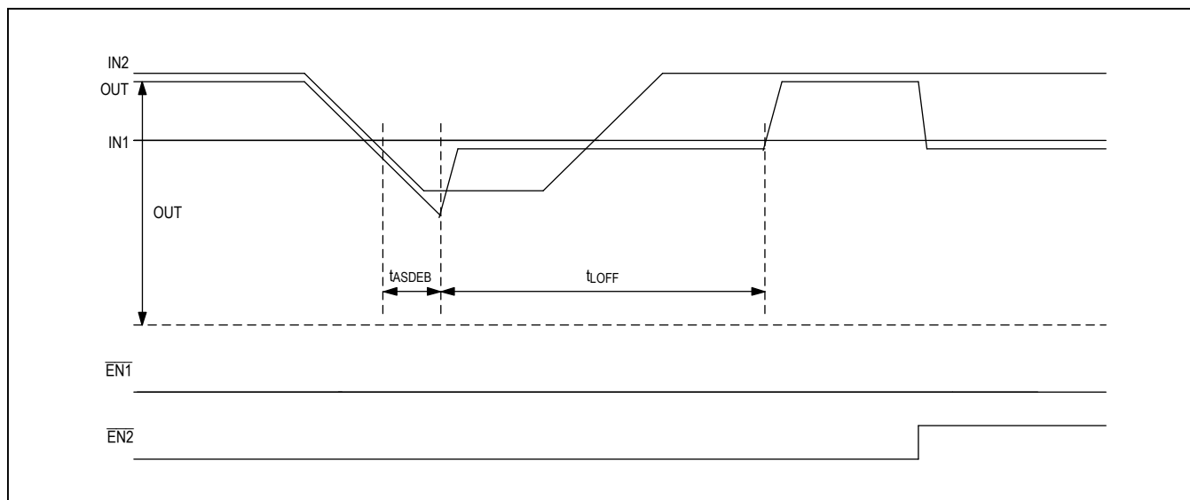
Figure 3: Automatic Switch Operation: IN2 Sag (Time scale is exaggerated for easy recognition in the waveform)
