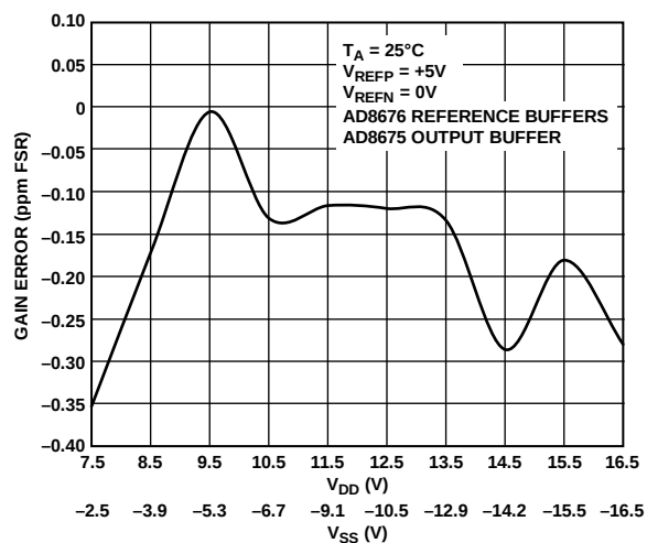
Figure 26. Gain Error vs. Supply Voltage, +5 V Span
