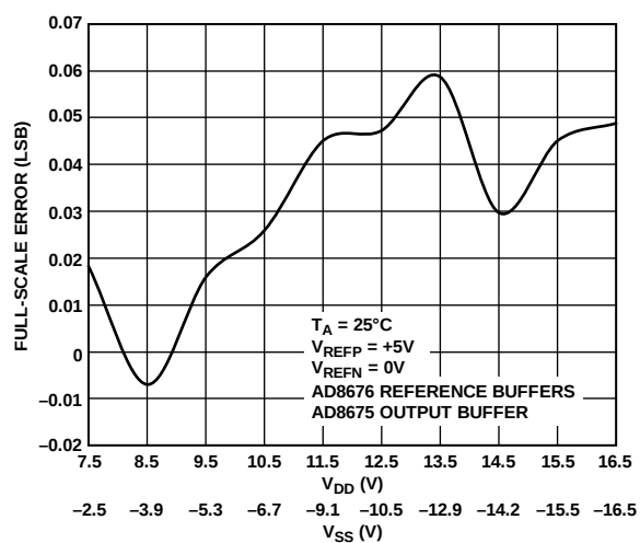
Figure 24. Full-Scale Error vs. Supply Voltage, +5 V Span
