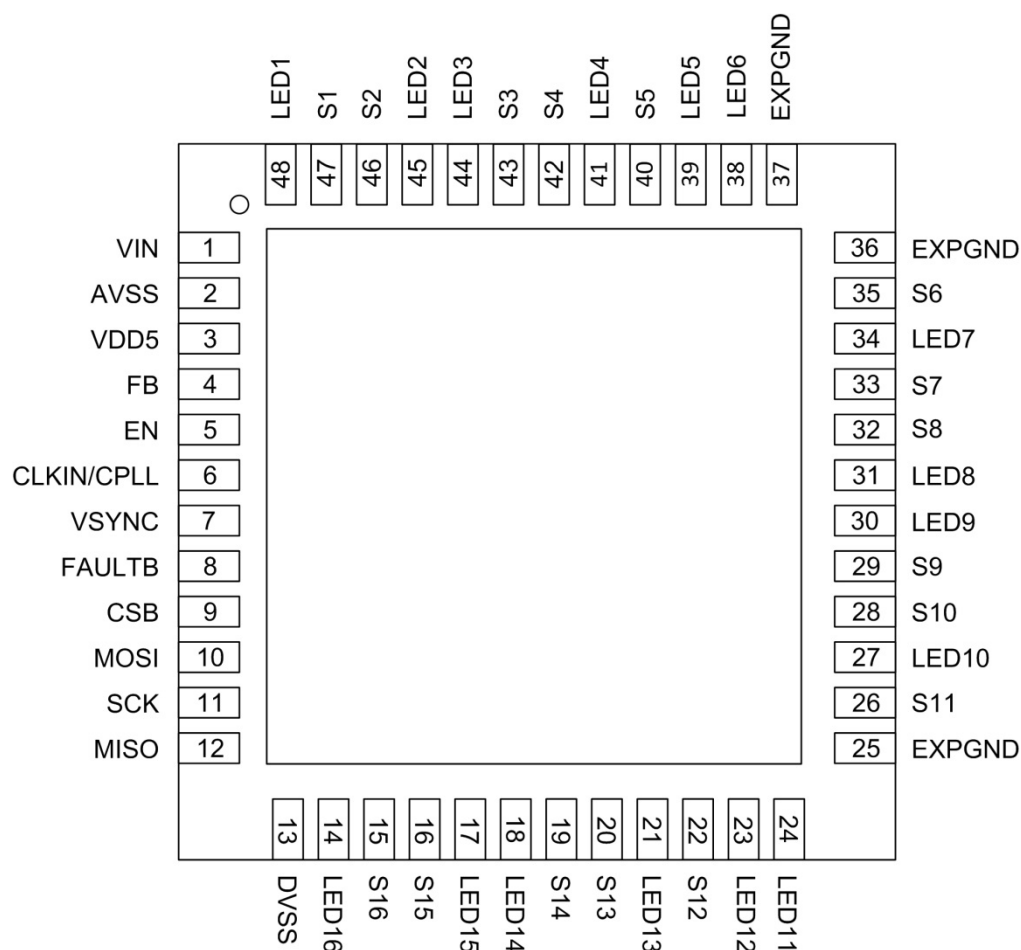
Figure 1.2: Connection Diagram
