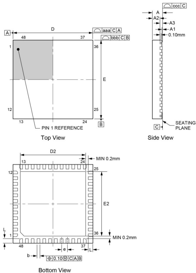
48-Lead QFN Package (7mm x 7mm)
