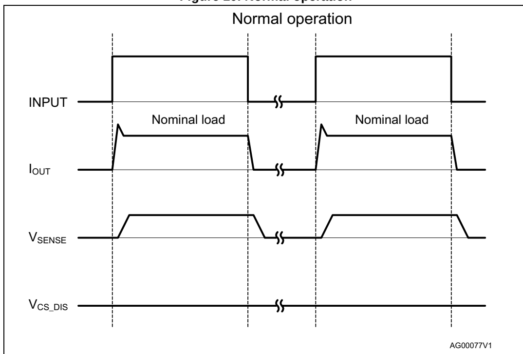
Figure 10. Normal operation
