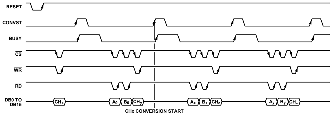
Figure 53. Software Parallel Mode Channel Conversion Setting
