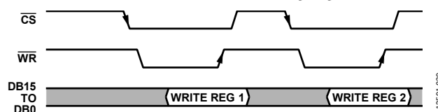
Figure 54. Parallel Interface Register Write
