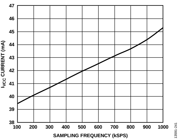
Figure 40. I_{VCC} Current vs. Sampling Frequency
