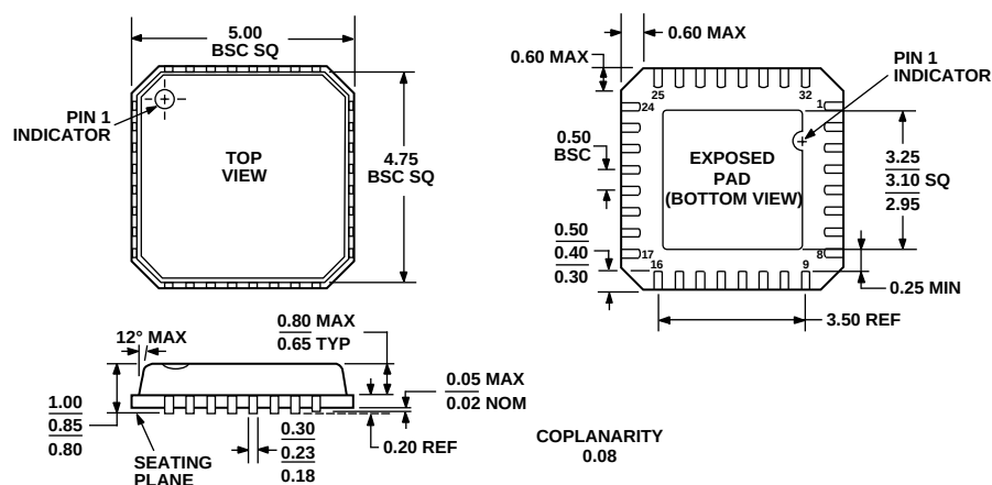
COMPLIANT TO JEDEC STANDARDS MO-220-VHHD-2 Figure 18. 32-Lead Lead Frame Chip Scale Package [LFCSP_VQ] 5 mm × 5 mm Body, Very Thin Quad (CP-32-2) Dimensions shown in millimeters
