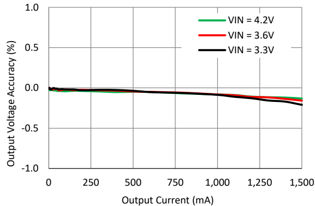
Output Voltage Accuracy vs Output Current
