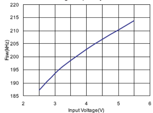
12. Switching Frequency
