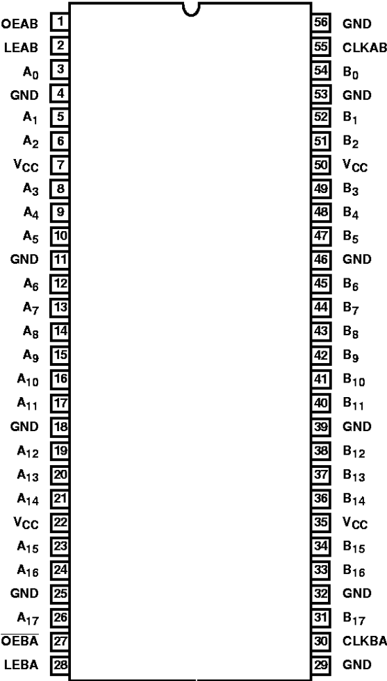
CD74FCT16501T, CD74FCT162501T, CD74FCT162H501T (SSOP, TSSOP) TOP VIEW
