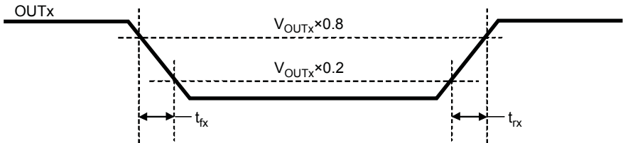
Figure 2. Output Switching Time
