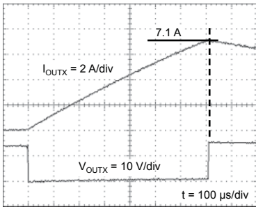
Low-side DMOSFET OCP Operation Example
