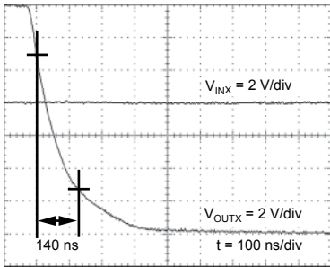
Output Fall Time, t_{FX}
