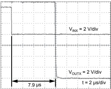
Input to Output Off Propagation Delay, t_{INX\_OFF}
